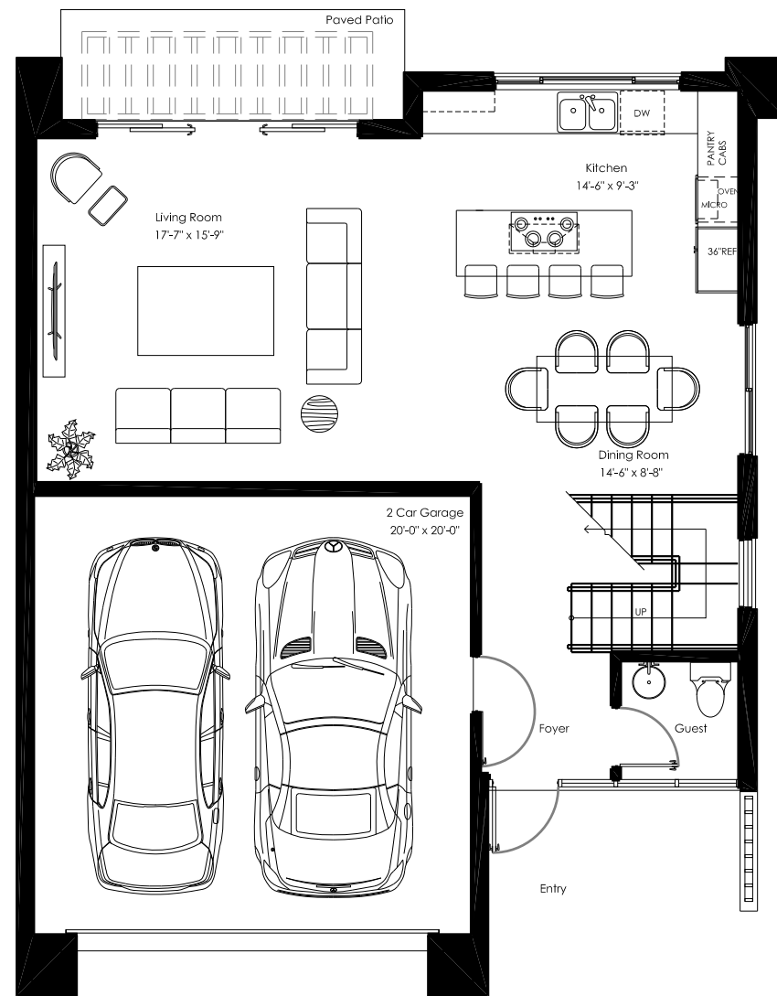
B1 FIRST FLOOR
